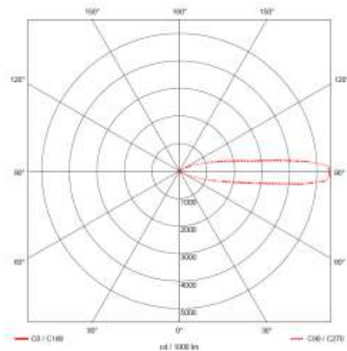
Figur 3: Spotlight beam characteristics
